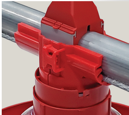
An anti-rotation clip* for tube programming holds the NutraPan feeder stationary on the feed tube.
