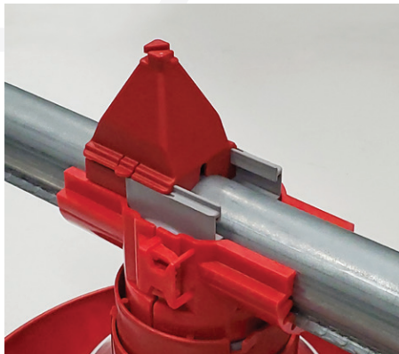
A 2-piece drop tube design allows for simple installation.
